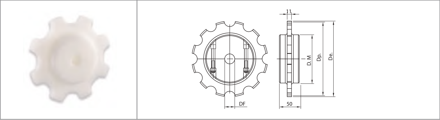
Split sprockets material: polyamide - screw in stainless steel - UNI 6604-69 key seat
