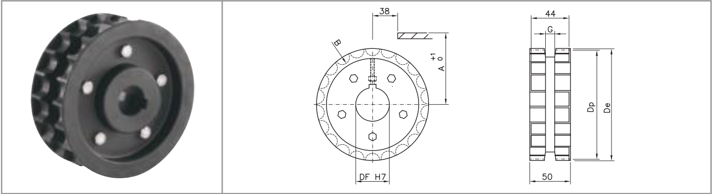
Standard sprockets material: reinforced polyamide - screws in stainless steel / UNI 6604-69 key seat
