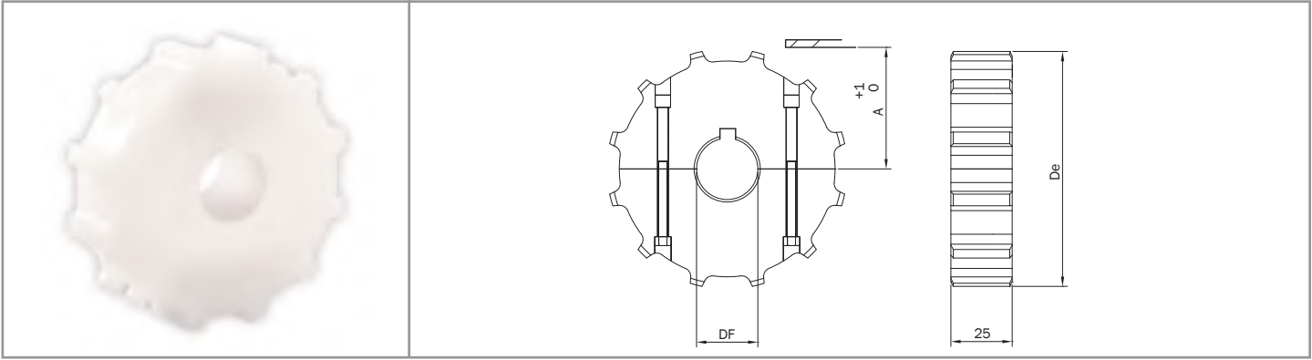
Split sprockets material: polyamide PA white - screw in stainless steel UNI 6604-69 key seat
