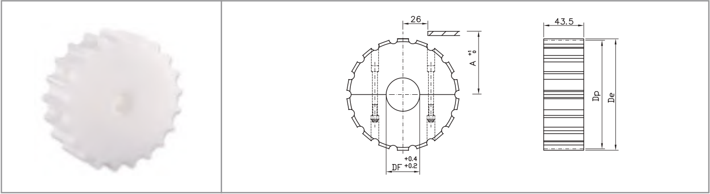
Split idler wheels material: polyamide - screws in stainless steel, nuts in zinc plated steel
