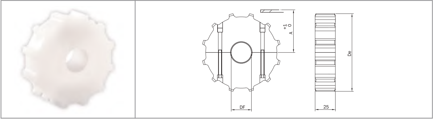
Split idler wheels material: polyamide PA white - screw in stainless steel
