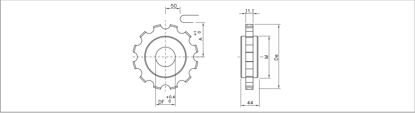
Standard sprockets material: zinc plated steel (Z), stainless steel (X)
