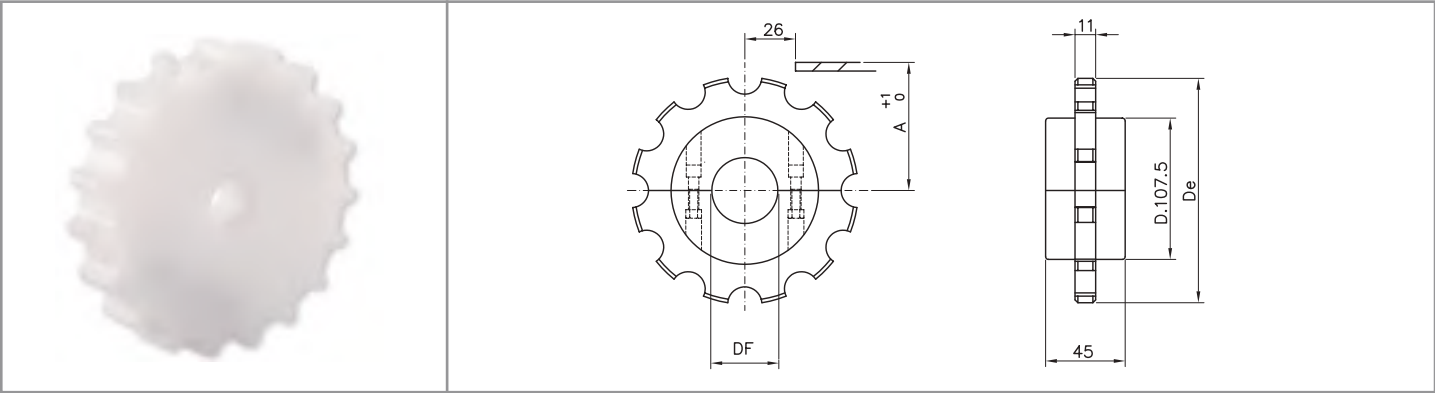
Split sprockets material: polyamide in PA white - screws in stainless steel
