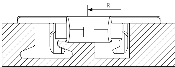
Series uni 879 Super Flex and 880 Super Flex, Carry section
