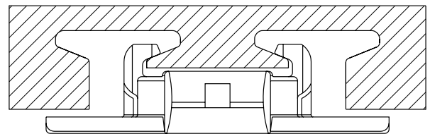
Series uni 879 Super Flex and 880 Super Flex, Return type
