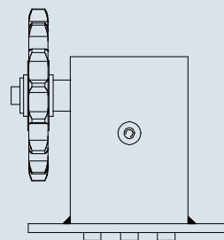
Spann-Box® size 1 with sprocket type K-S – page 148
