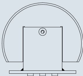
Spann-Box® size 1 with return profile – page 146
