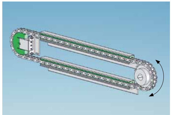
Return/tensioning station
