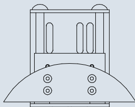
Spann-Boy® TS with arc segment profile – page 139
