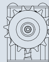
Spann-Boy® with sprocket page 138
