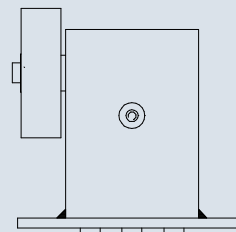
Spann-Box® size 1 with tensioning roller type SR-S page 159
