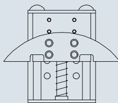
Spann-Boy® with arc segment profile – page 137
