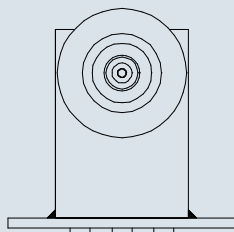
Spann-Box® size 1 with tensioning roller type SR-L page 158
