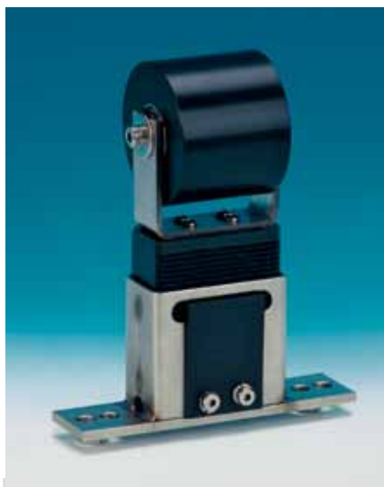
Spann-Box® designs with locking devices; they prevent the slide profile from being compressed when the direction of rotation changes, for example.
