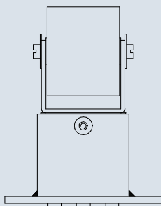
Spann-Box® size 1, belt tensioner with tensioning roller at top page 157
